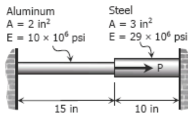
Figure P-273 and P-274
