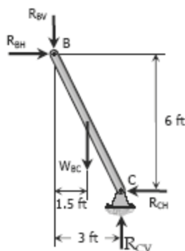
FBD of member BC
