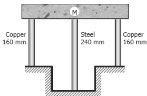
Figure P-236 and P-237
