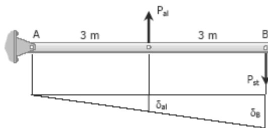
FBD and movement diagram of bar AB
