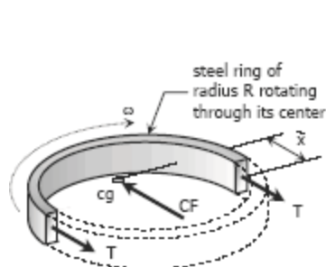
FBD of Ring in Rotation
