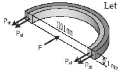
FBD for p \geq 2.381 \text{ MPa}
