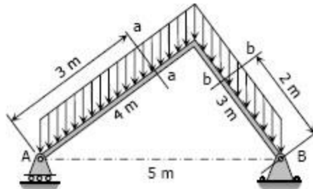
Figure P-514 and P-515
